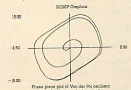
Phase plane plot of Van der Pol oscillator (ms = x horizontal, y vertical)
